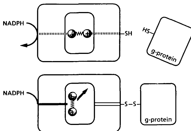
Figure 7 Influence of scattering group orientation on electron tunnelling. Scattering from a dipolar group with a clearly defined direction of charge movement will cause the electrons to change direction as well as energy. If the dipole movement is parallel to the tunnelling path (top) the electrons will continue in a straight line. If the dipole oscillates at right angles to the tunnelling path, electrons will be scattered sideways. In this schematic the donor and acceptor sites are arranged in such a way that electrons scattered transversely do not reach the acceptor site, and therefore cannot reduce the disulphide bridge to effect G-protein transduction
