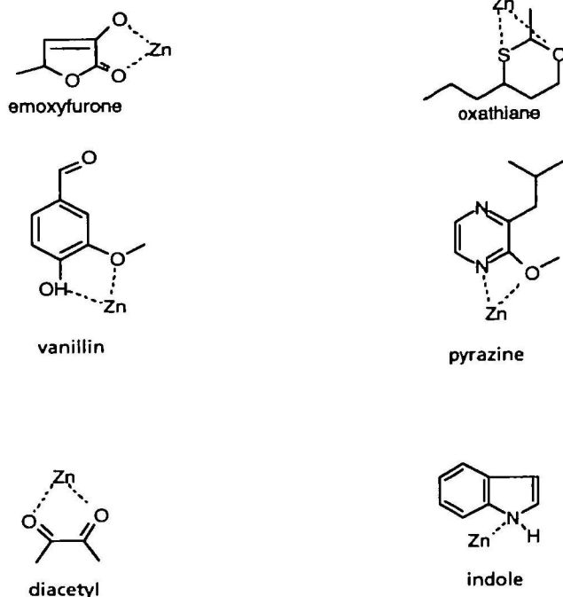
Figure 12 Six exceptionally strong odorants, showing that they share the ability to coordinate to a zinc ion. See text.
