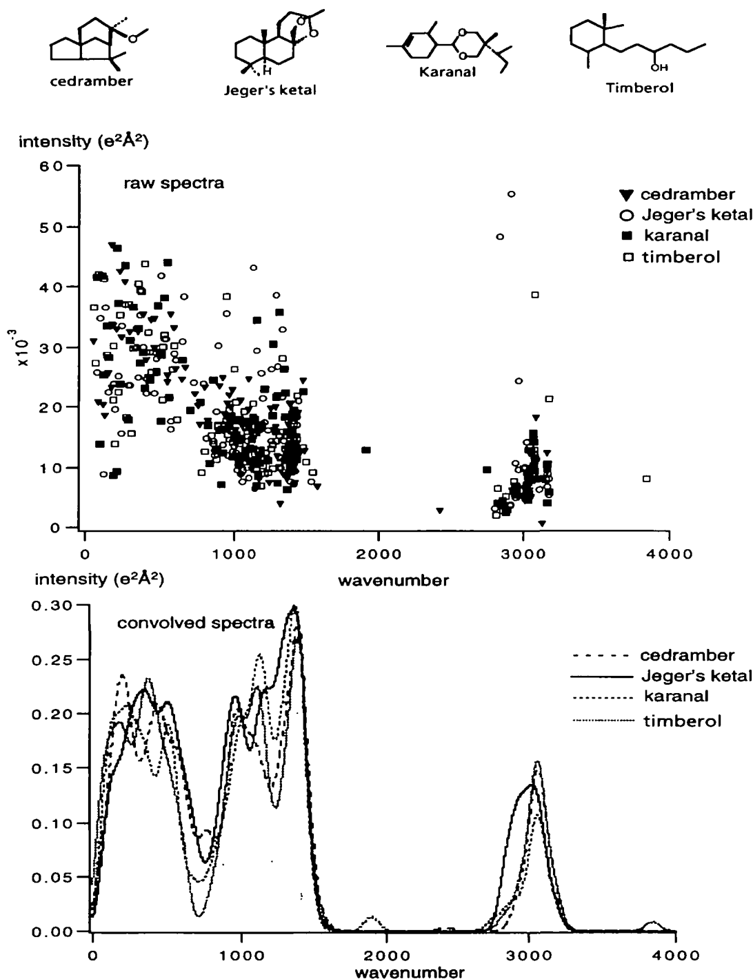
Figure 5 Structures (top), raw vibrational spectra from CHYPRE calculations (middle) and convolved spectra (bottom) for four ambergri odorants with closely related odours and very different structures. Each point in the raw spectra represents the energy and amplitude of a single vibrational mode. A considerable degree of scatter is present, reflecting the structural diversity of the molecules. By contrast, the convolved CHYPRE spectra, like the odours, are remarkably similar.
